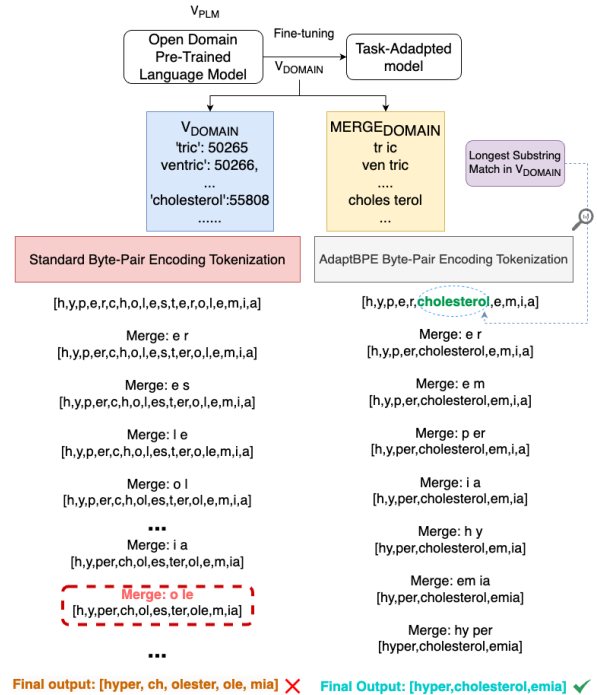
Figure 1: ADAPT-BPE modifies the initialization step of standard BPE by merging the characters that match with the extended vocabulary ( V_{\text{DOMAIN}} ). The incorrect merge step of BPE for tokenizing the word hypercholesterolemia is highlighted by a red dashed box.
