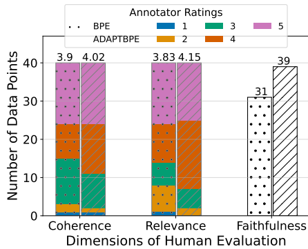
Figure 2: Human evaluation scores comparison over 40 randomly selected test data points. ADAPTBPPE produces more relevant, coherent, and faithful summaries during human evaluation with medical experts.
